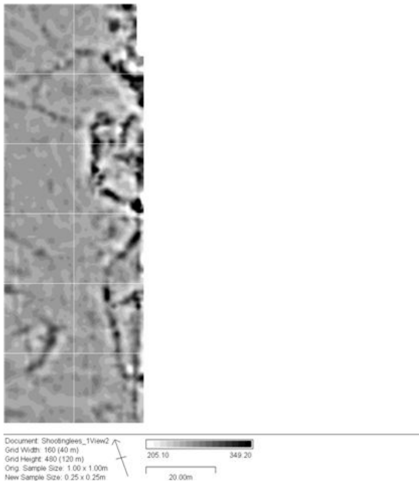
Fig 1 Resistivity Survey
